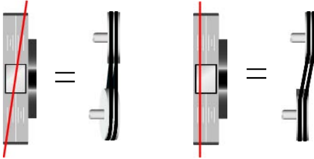
Observed Axial offset
